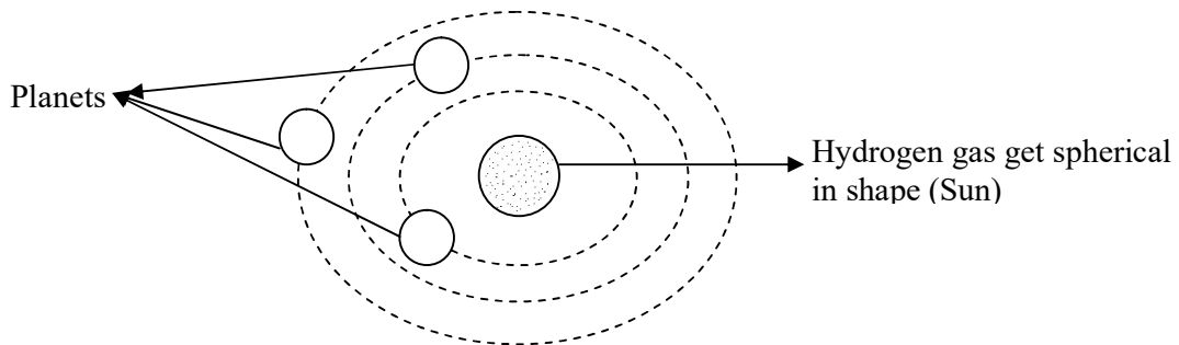
After getting gravitational force (sun family)
